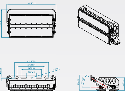
MF-FLL480WB
