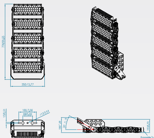
MF-FLL600WA
