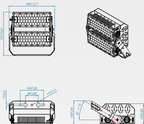
MF-FLL240WA
