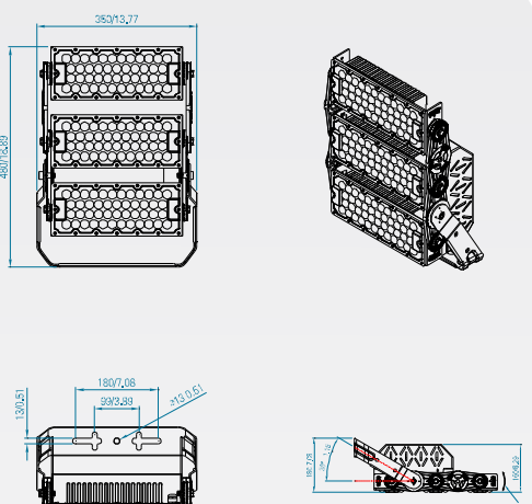
MF-FLL360WA
